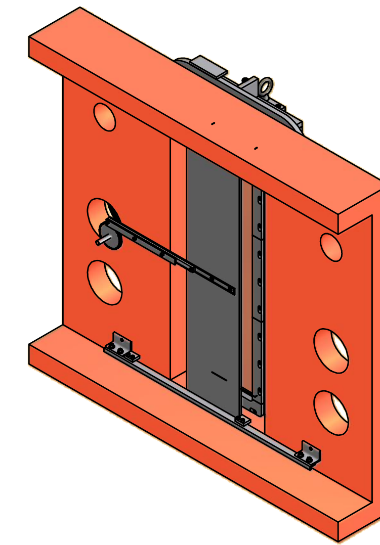
ISOMETRIC SCALE 1/8
